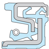
Simmerring® Cassette seal type 3
